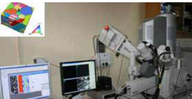
▼ Orientation Imaging Microscope Facility
