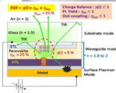
▲ Improving perovskite LED Efficiency
