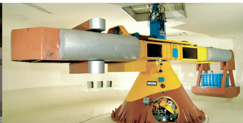
▼ Sudarshan: The National Geotechnical Centrifuge Facility
