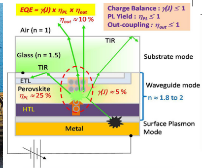
▲ Improving perovskite LED Efficiency
